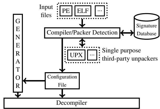
Figure 1. Preprocessing scheme. [3]
