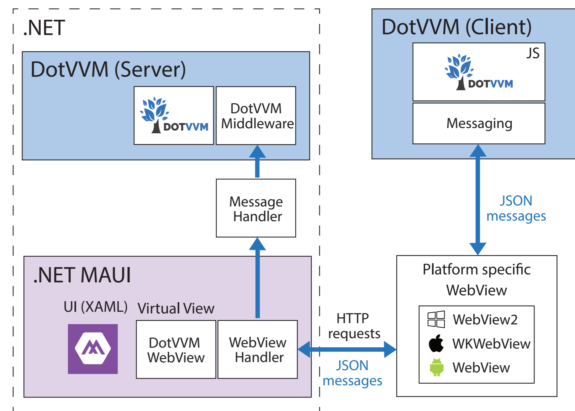
Figure 1: Communication between DotVVM and .NET MAUI using WebView.
