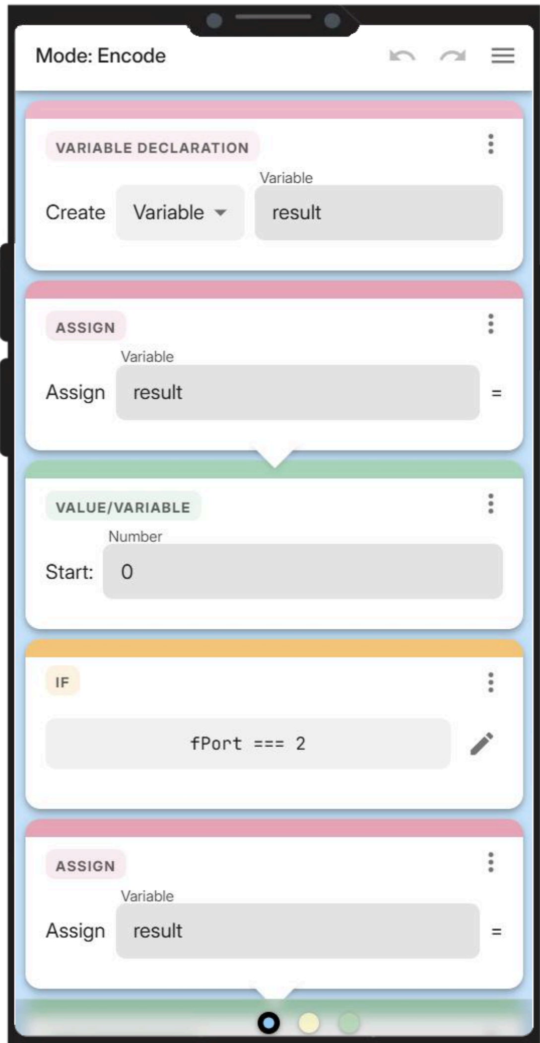
Figure 1: Program Example
