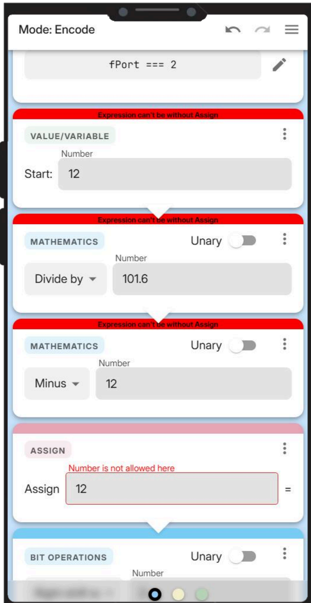
Figure 3: Validation
