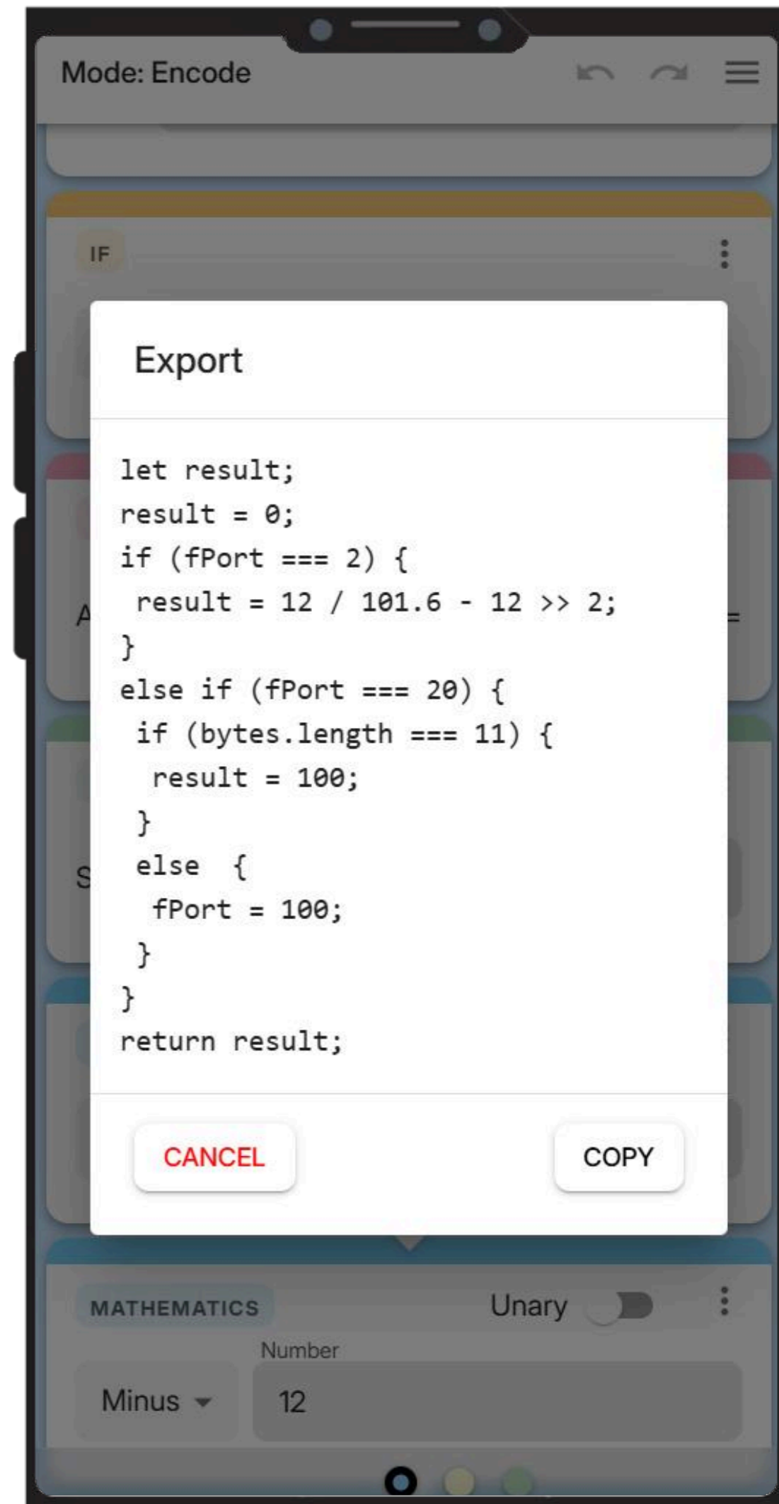
Figure 2: Code Generation
