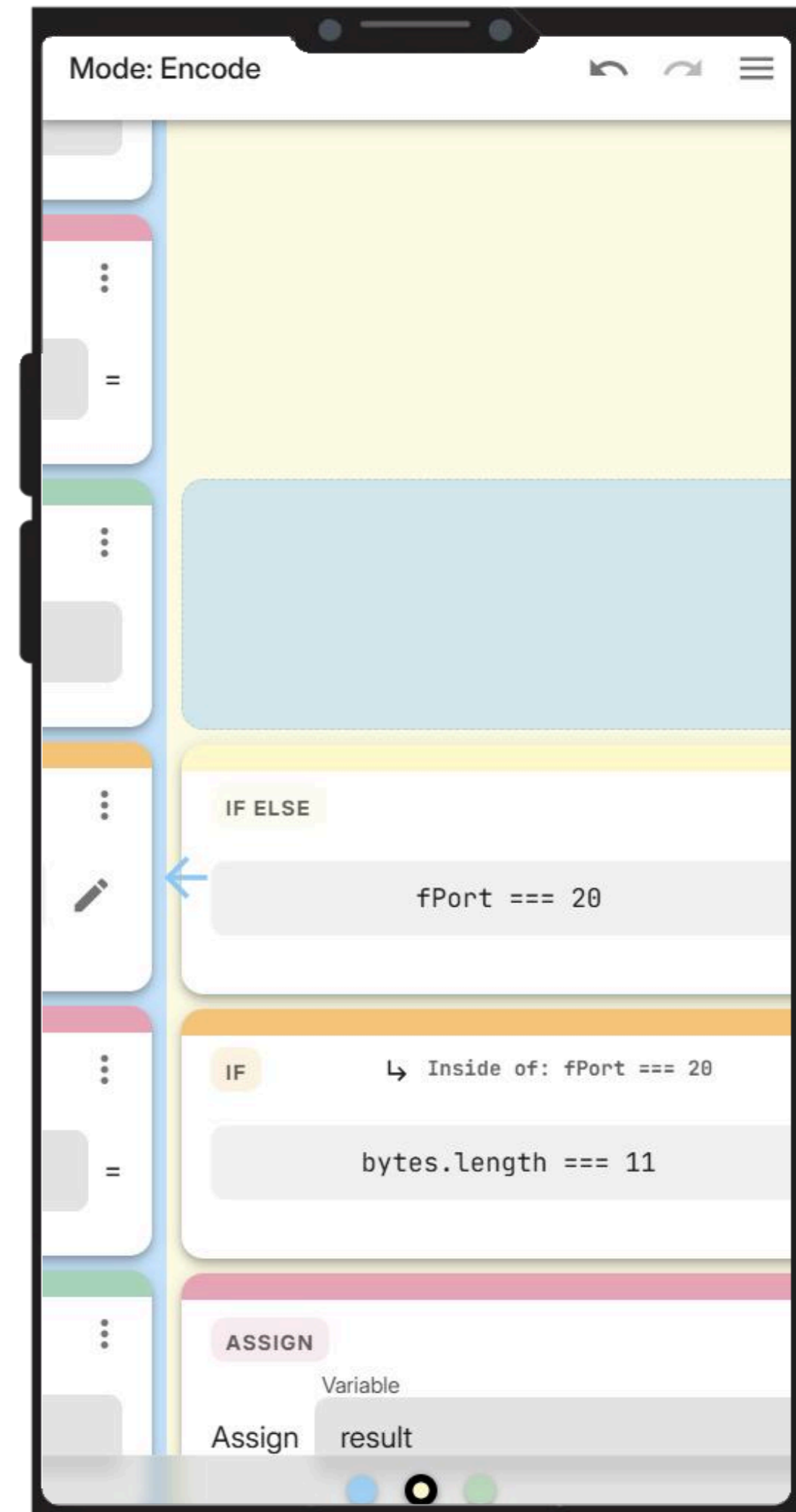
Figure 4: Swiping & Branches
