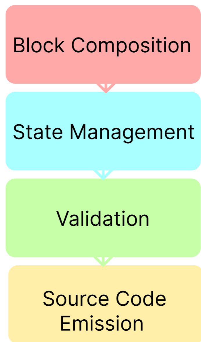
Figure 5: Creation Pipeline
