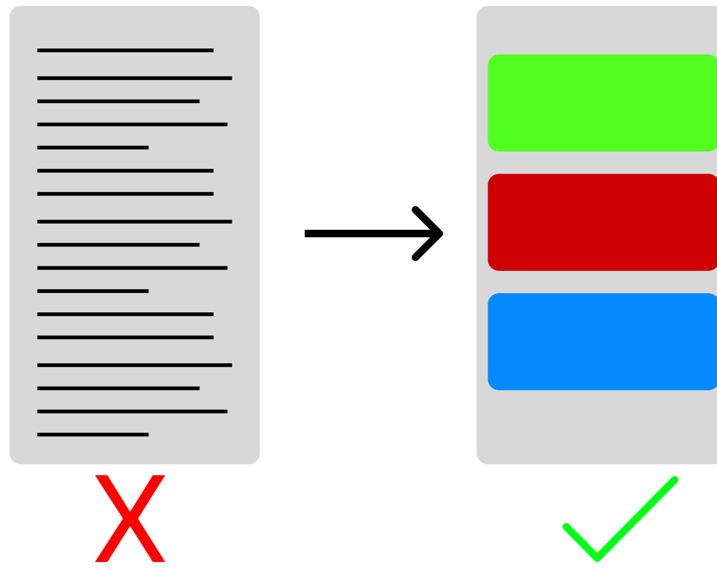
Figure 6: Motivation
