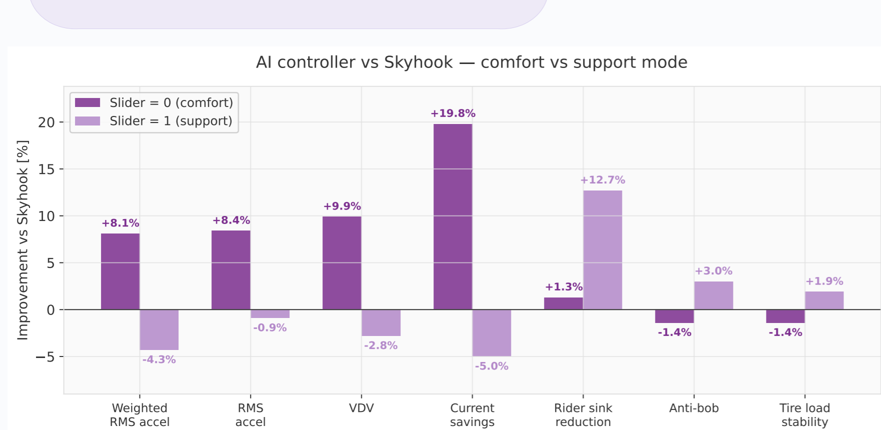
Fig. 4: Controller comparison
