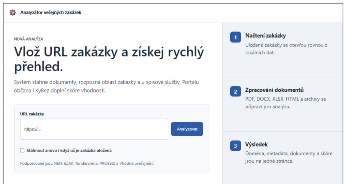
Figure 3: Input interface for submitting a tender URL
